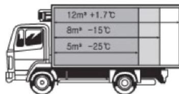
Selection Guide(Ambient 38℃)
